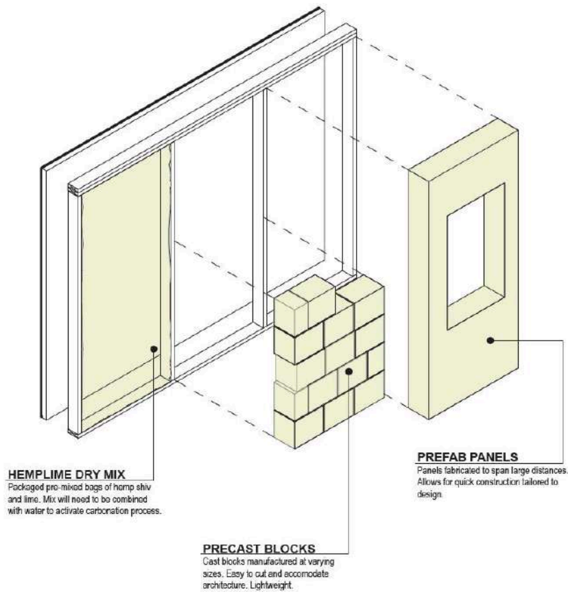
Diagram hemp and lime wall systems
