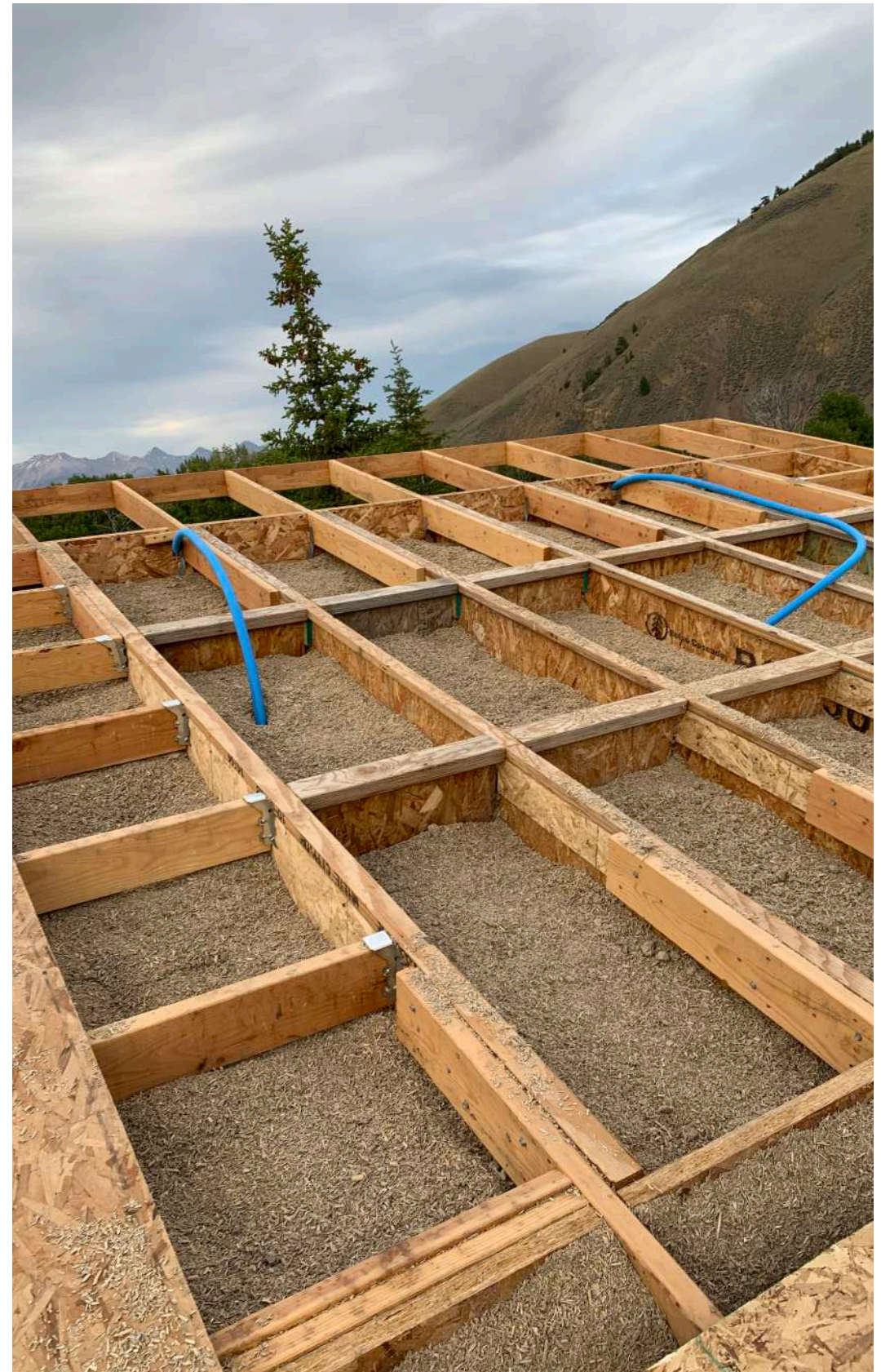
Fig 7.4 Floor fabrication
