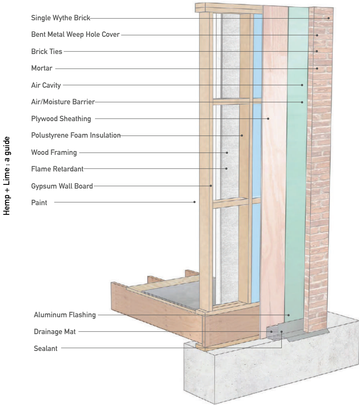
Fig 7.5 Brick Veneer Wall Section
