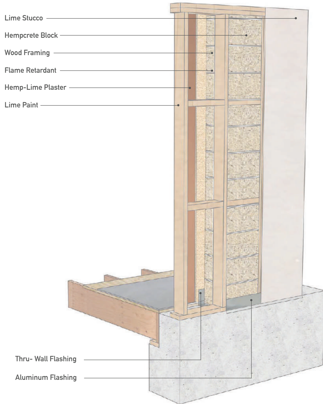
Fig 8.0 Hemp+Lime Wall Section
