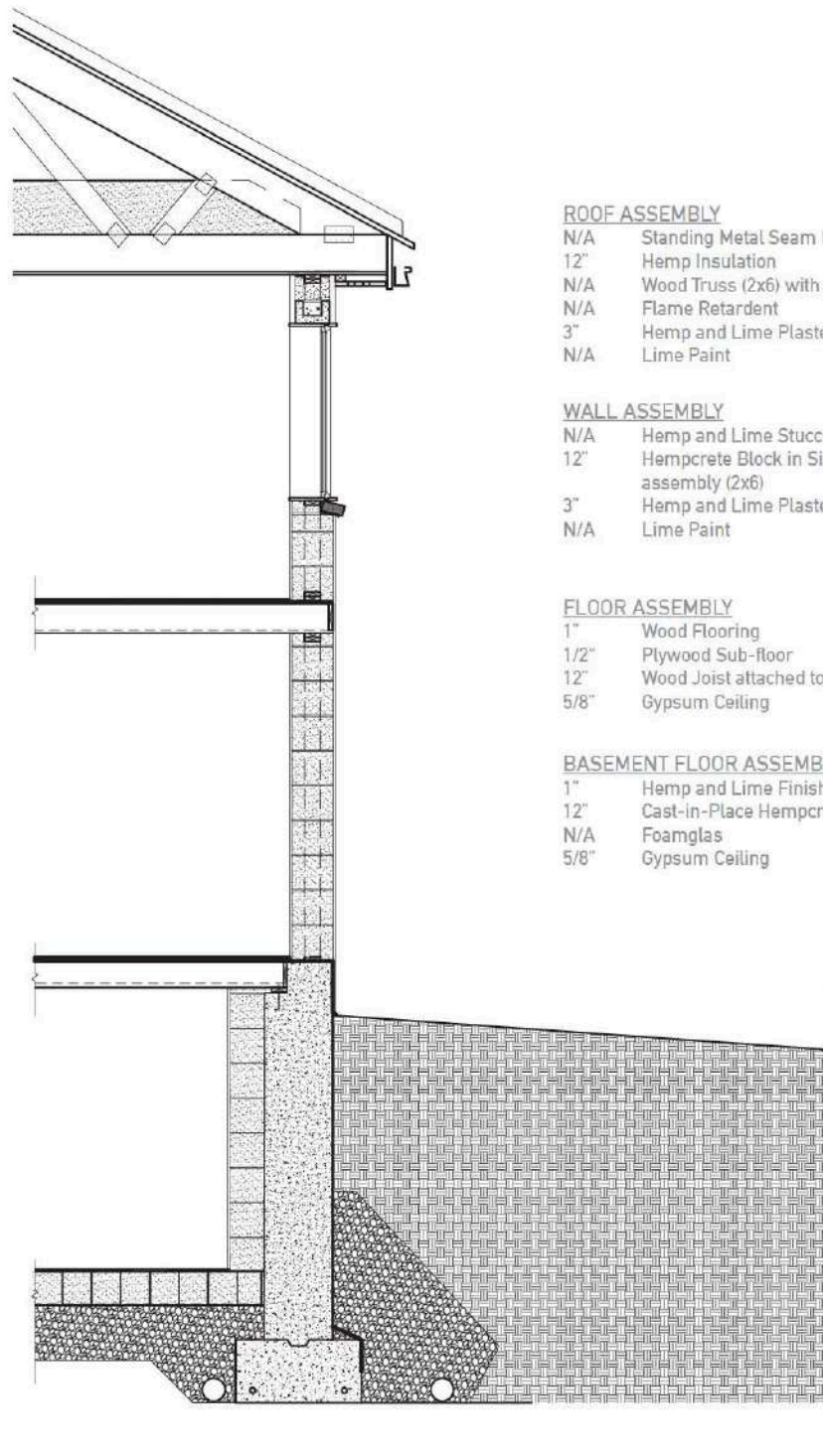
Fig 8.1 Typical Wall Section: Hemp+Lime Construction
