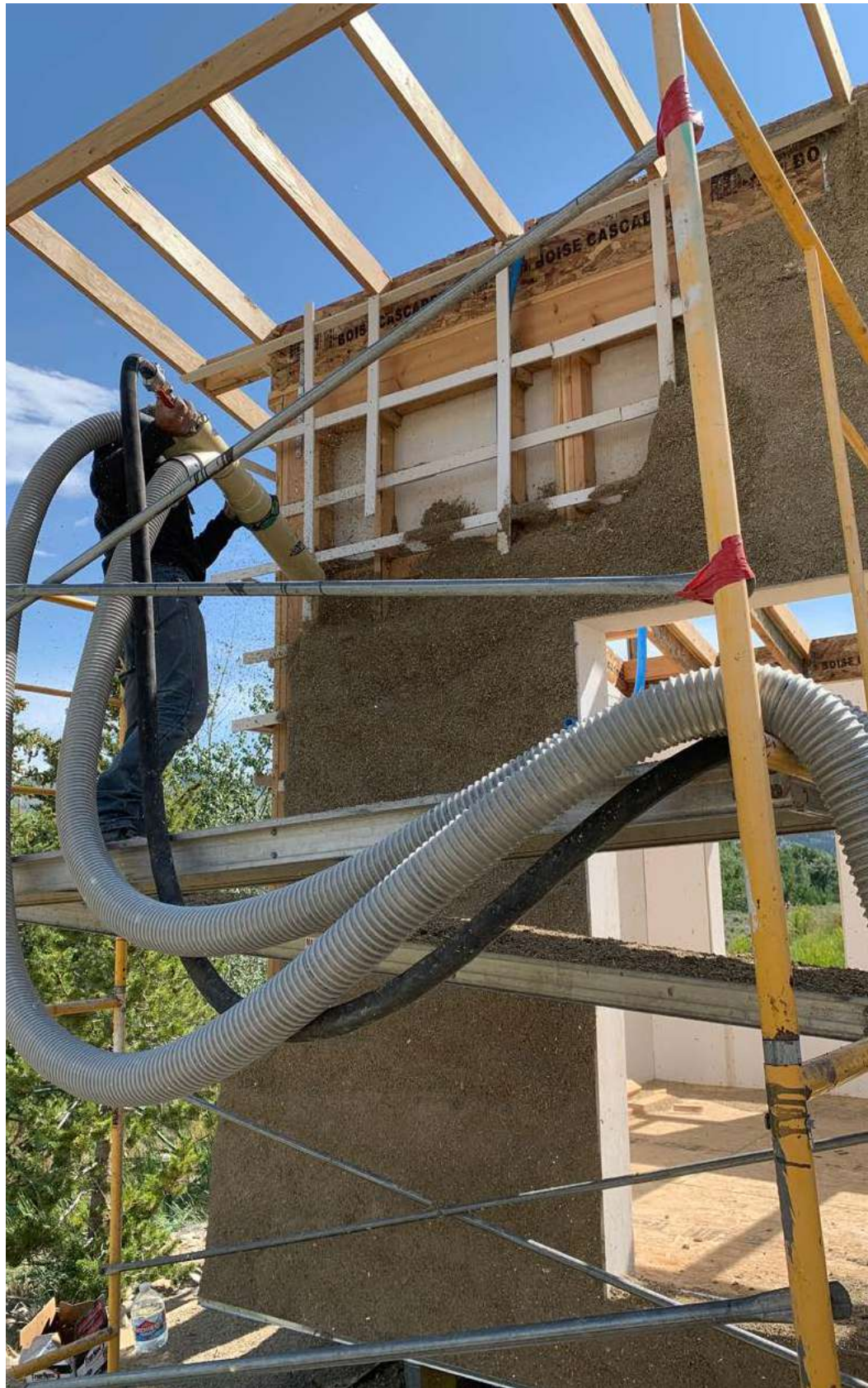
Fig 7.3 Blown system for cast in place hemp+lime construction
