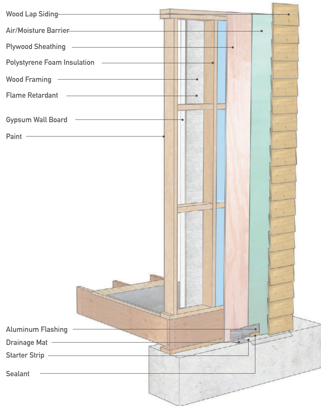
Fig 7.7 Wood Clapboard Wall Section
